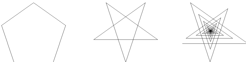
Figure 6: A pentagon, a five pointed star, and a spiral generated by the programs in Table 1. Here the spiral angle A = 4\pi / 5 and the scale factor for the spiral is S = 9/10 .
