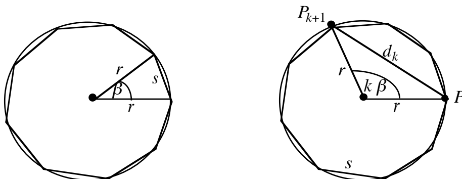
Figure 11: The Law of Cosines provides a relationship between the length of a side and the distance from a vertex to the center of a regular polygon (left). Similarly, the Law of Cosines provides a relationship between the distance from a vertex to the center of a regular polygon and the length of each diagonal of the polygon. Notice that if the polygon has n sides, then \beta = 2\pi / n .
