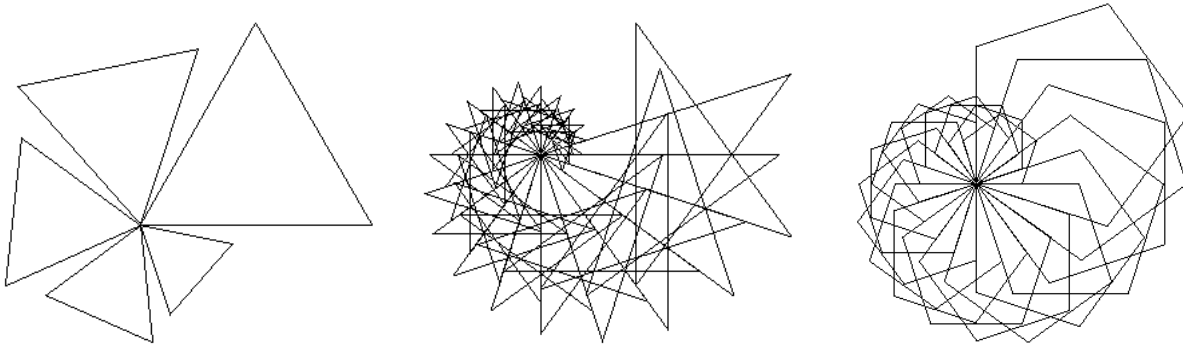
Figure 10: The effect of composing SPIN with SCALE: starting with a triangle (left), a star (center), and a pentagon (right).
