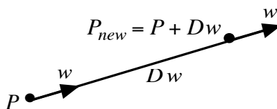
Figure 3: The command FORWARD D changes the turtle's location, but leaves her direction and step size unchanged. The new turtle location is:
