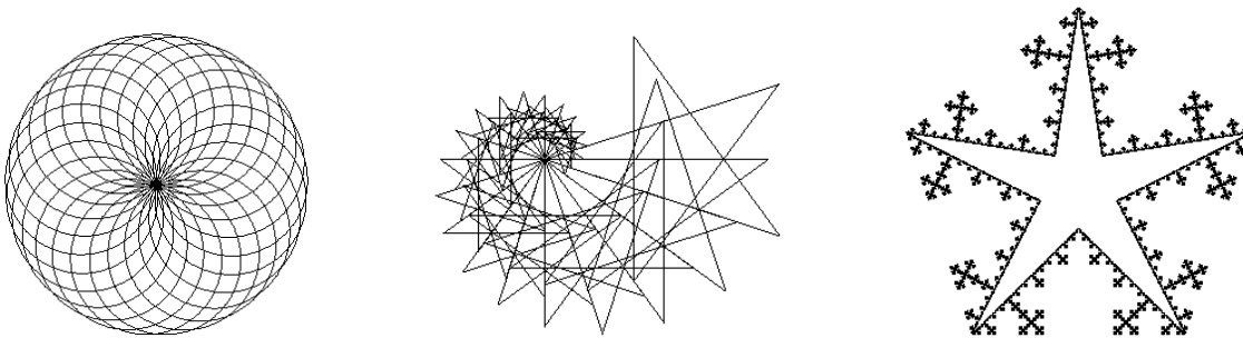
Figure 1: Some interesting geometric patterns generated by turtle paths.
