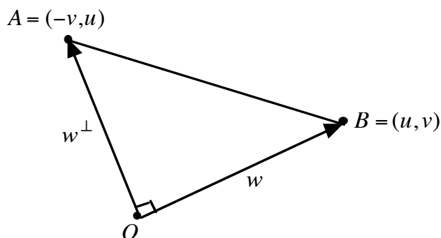
Figure 12: The vectors w = (u, v) and w^\perp = (-v, u) form a right angle at the origin O .
