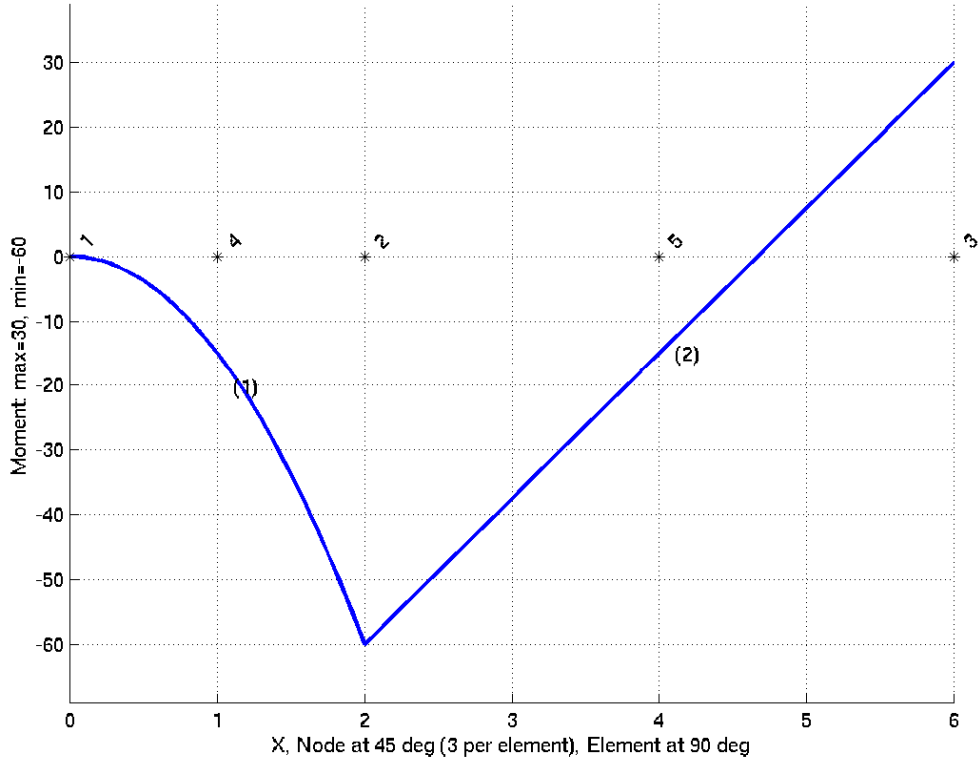
Quintic Beam Moment from: 2 Elements, 5 Nodes
