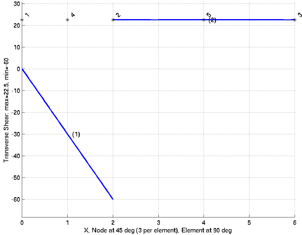
Quintic Beam Shear from: 2 Elements, 5 Nodes
