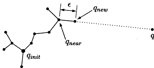
Figure 3: The EXTEND operation.
