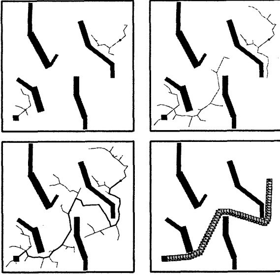
Figure 6: Growing two trees towards each other.
