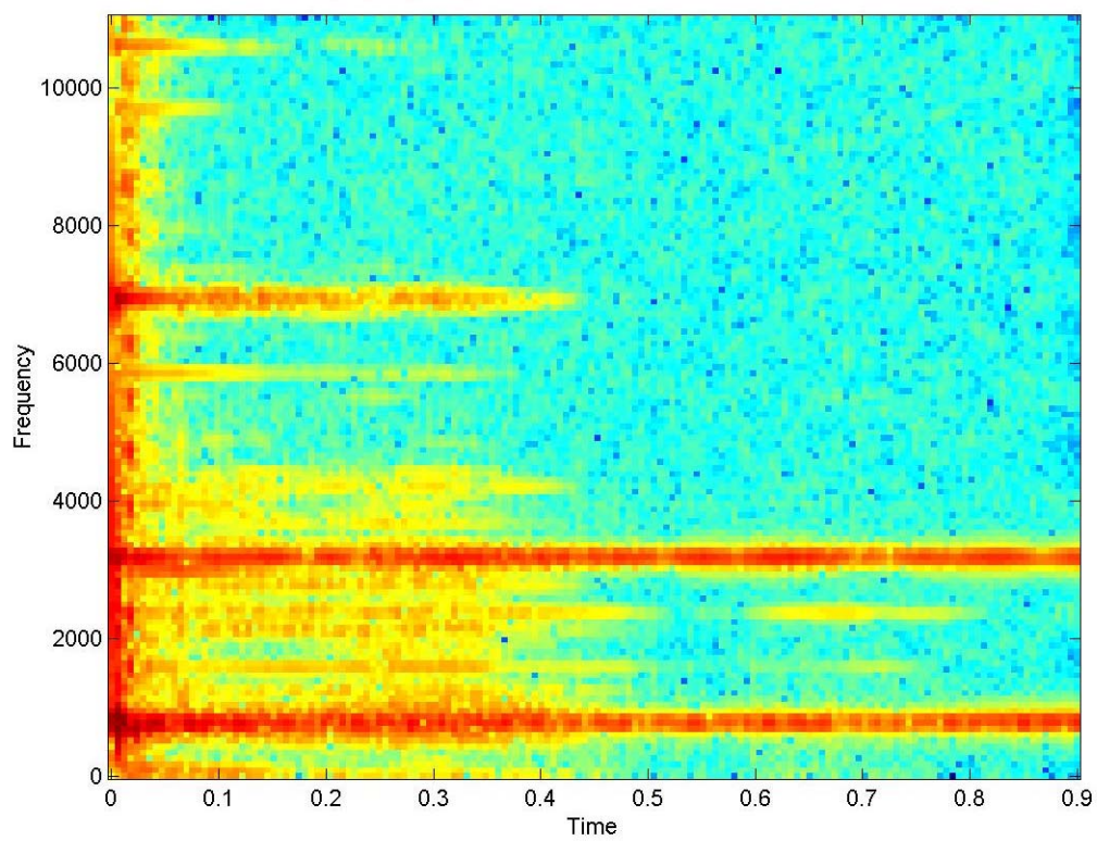
DING.wav after keeping only frequencies within 3 stds from the mean
