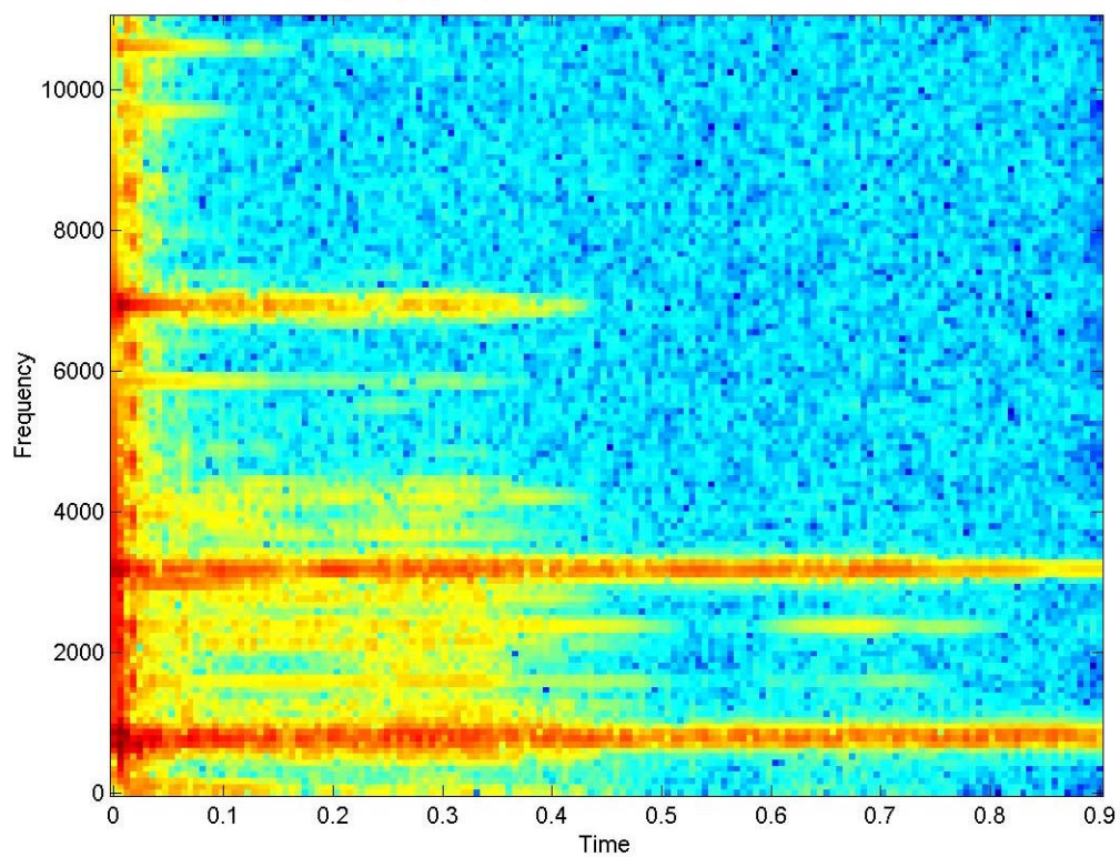
DING.wav after only keeping frequencies within 2 stds from the mean
