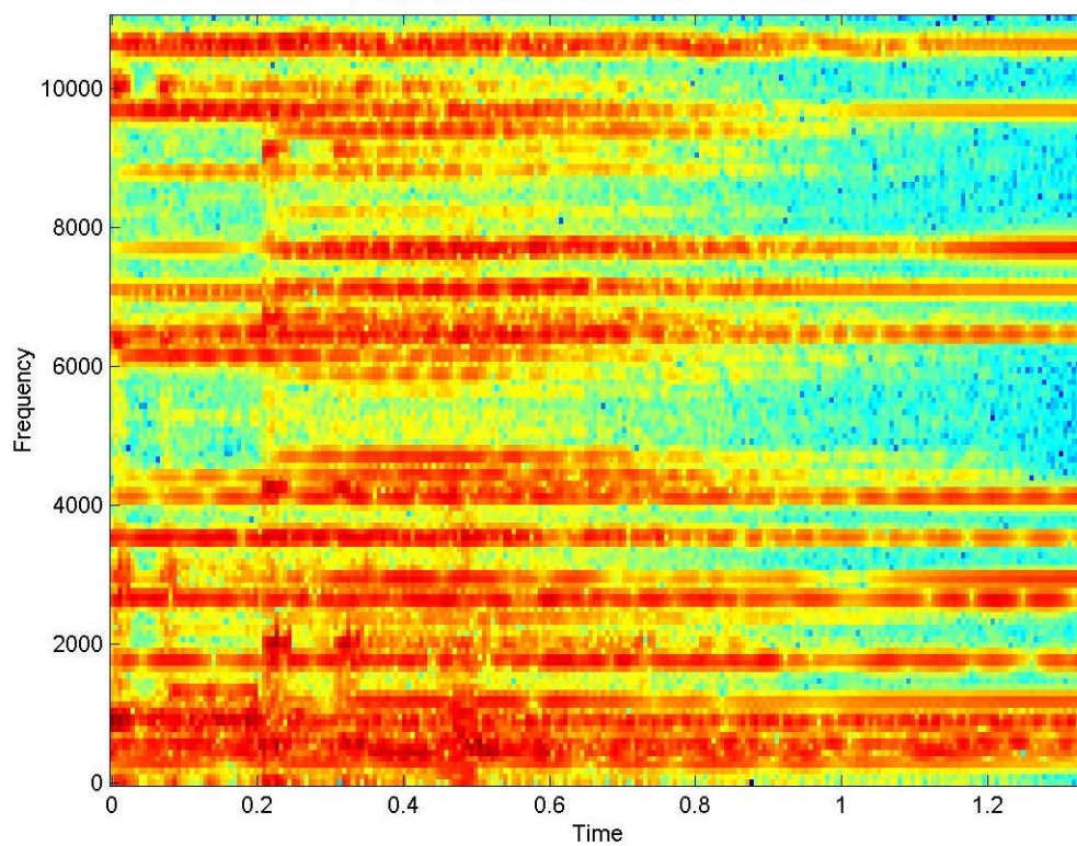
NOTIFY.wav after only keeping frequencies within 2 stds from the mean
