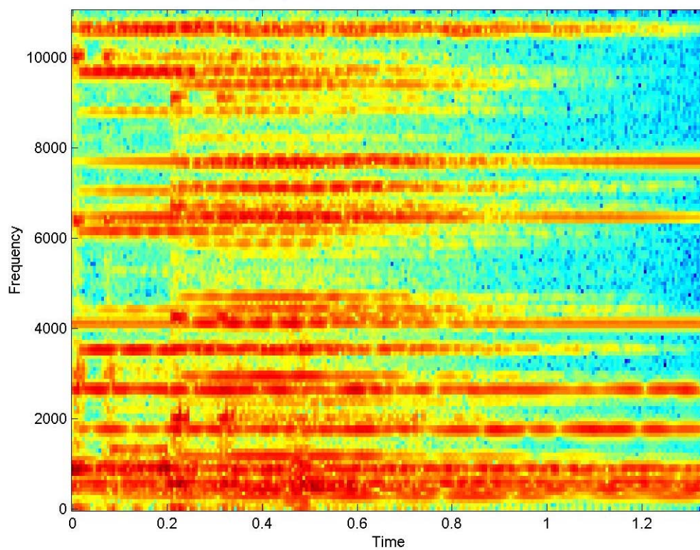
NOTIFY.wav after keeping only frequencies within 3 stds from the mean
