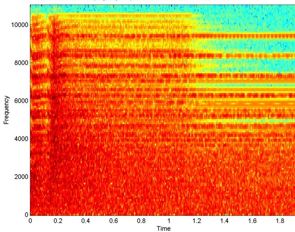
TADA.wav after keeping only frequencies within 3 stds from the mean
