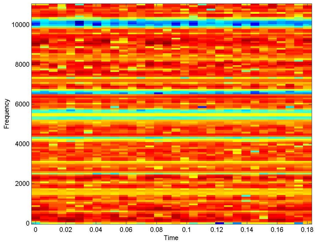
Utopia Open.wav after keeping only frequencies within 3 stds from the mean
