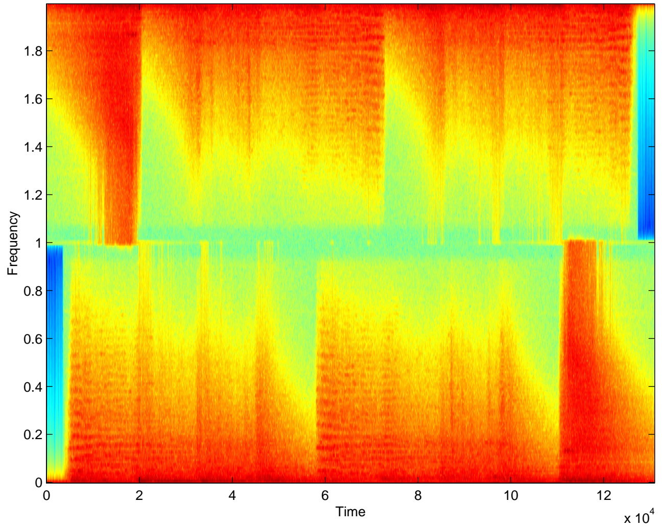
Spectrogram of "Classical", odd samples dropped
