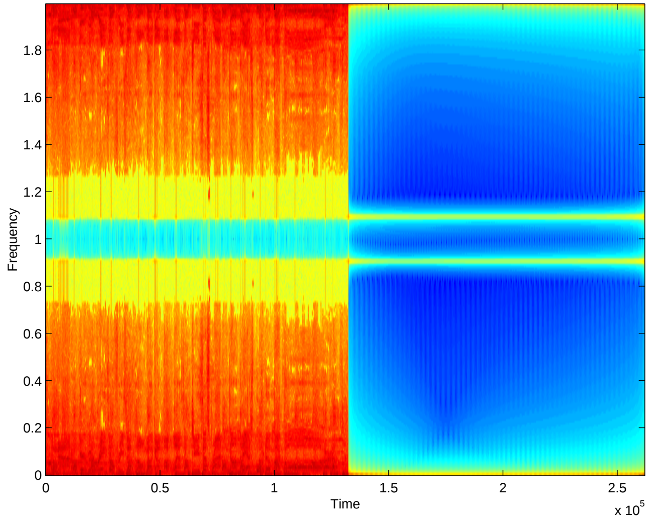
Spectrogram of "Plastic Jesus", <20Hz, >20kHz removed
