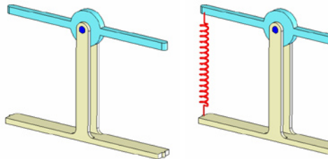
FIGURE 15: THE SWING ARM ON THE LEFT CAN MOVE WITHOUT DEFORMATION; THUS IT'S A MECHANISM. ANY MOVEMENT IN THE ARM ON THE RIGHT IS ACCOMPANIED BY DEFORMATION OF THE SPRING; THIS MEANS IT'S A STRUCTURE.
