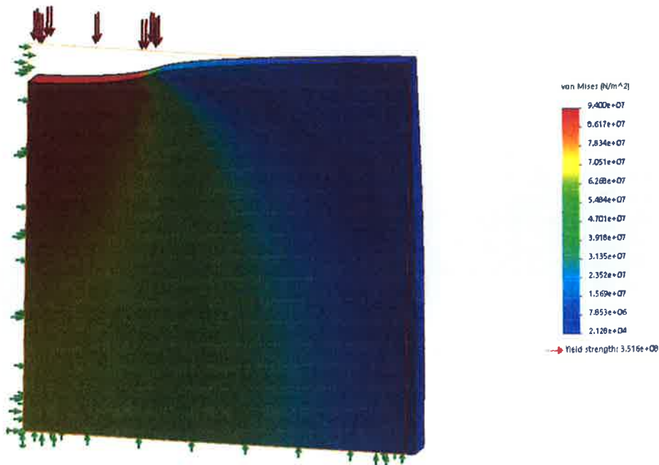
Figure 3: Von Mises Stress
