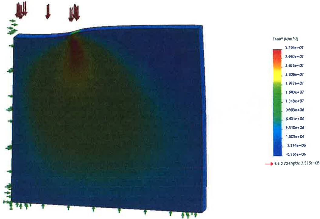
Figure 2: XY Shear Stress
